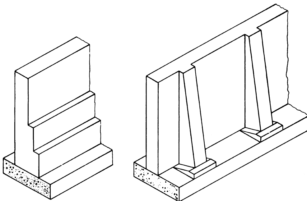
Figure 14 — Stepped and buttressed retaining walls in unreinforced masonry
