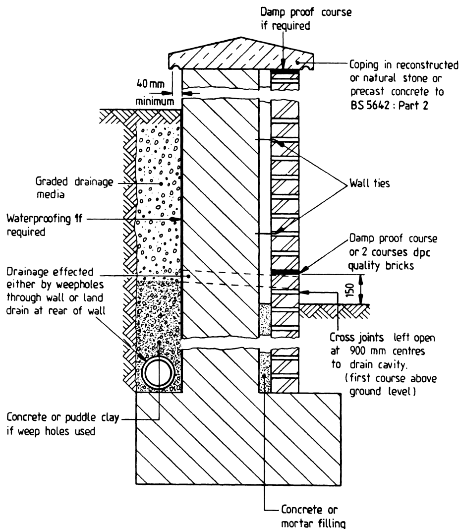
Figure 13 — Masonry clad mass concrete wall with cavity
