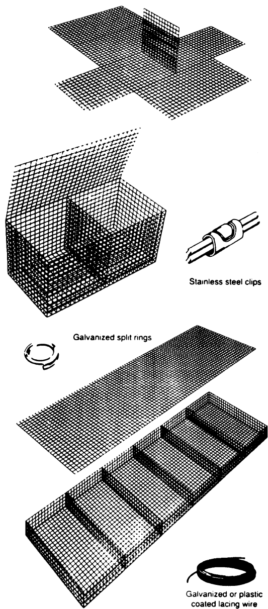
Figure 16 — Welded mesh gabion cage (typical)
