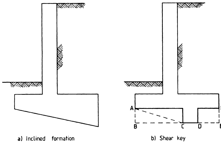
Figure 11 — Foundations of gravity walls
